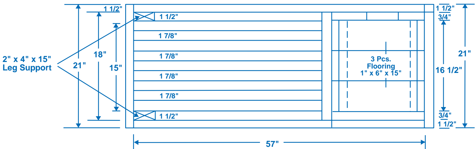
SIDE VIEW
